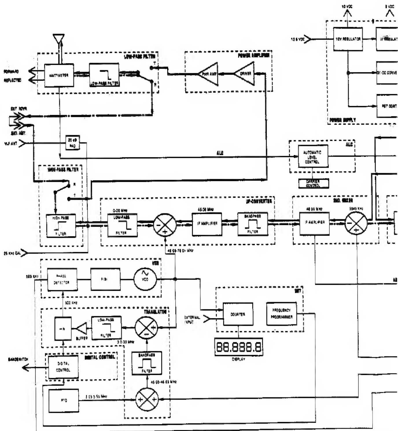
BLOCK DIAGRAM TRK HIGBAND
