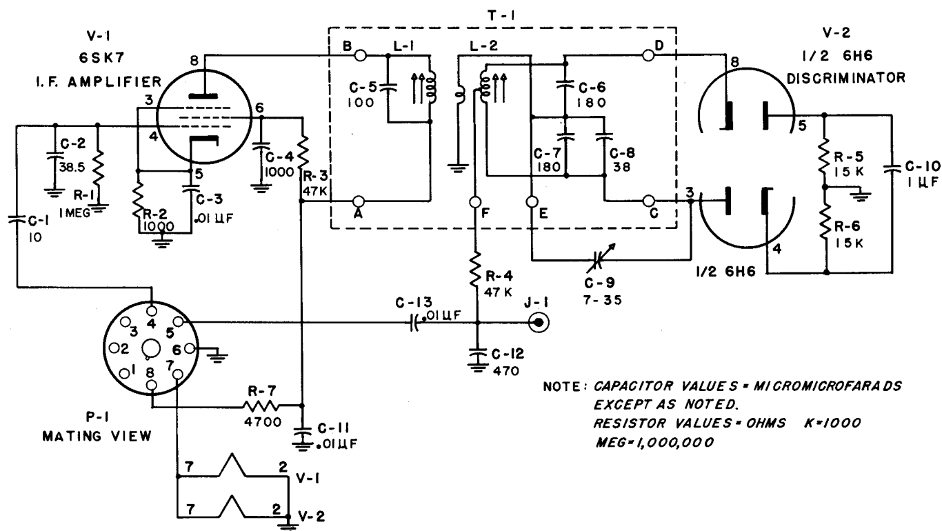
Figure No. 14. Schematic Diagram, NFM-83-50 Adaptor
