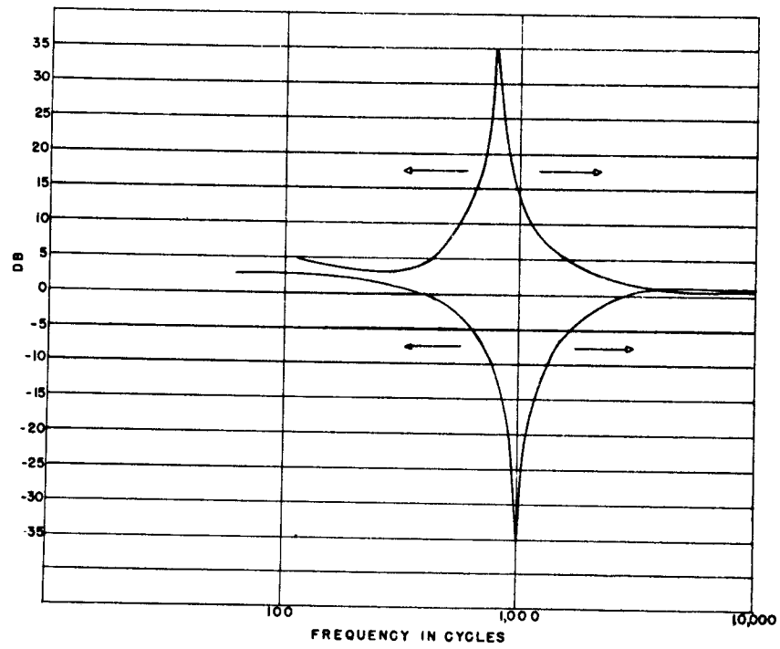
Figure No. 16. Characteristic Curve of Select-O-Ject Performance
