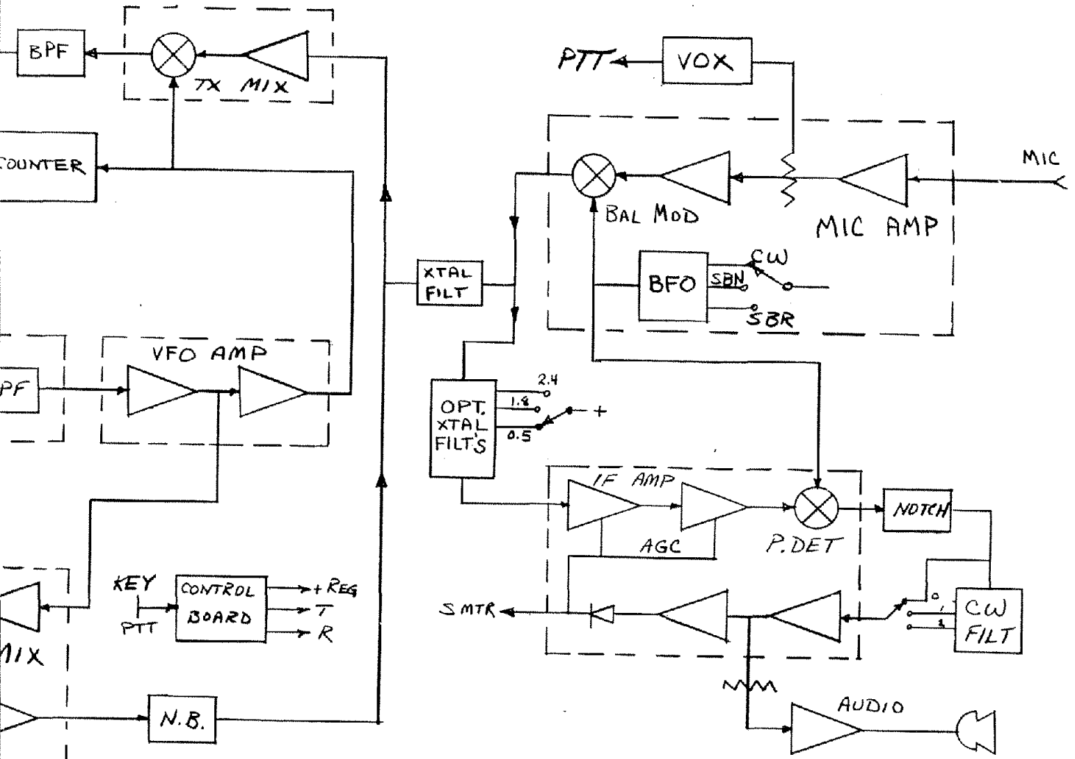
IS PATHS OMNI SIGNAL BLOCK DIAGRAM
