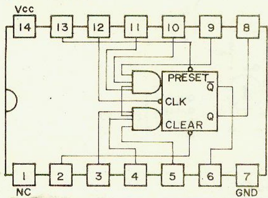
Internal Block Diagram of I.C.
