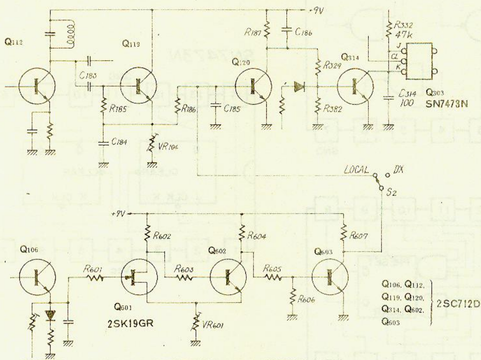
Scan Locking Circuit
