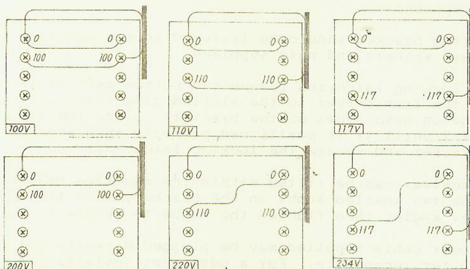
Transformer Rewiring
