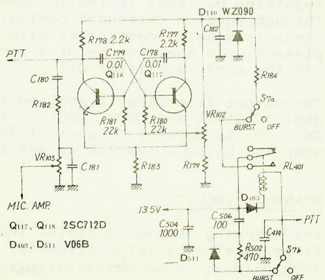
Burst Circuit
