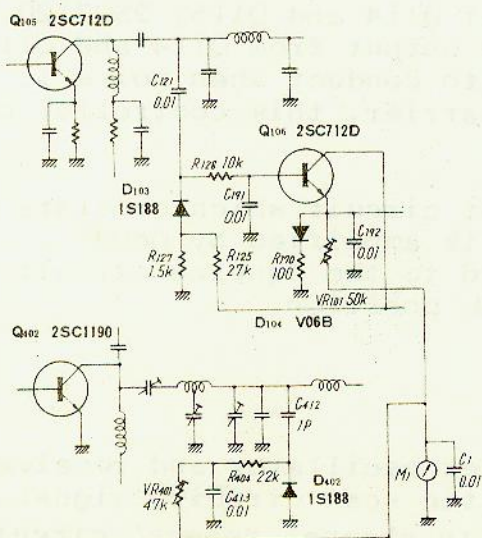
Meter Circuit
