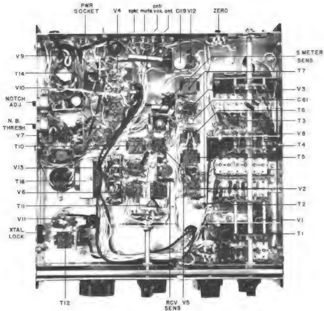
FIGURE 10 BOTTOM VIEW
