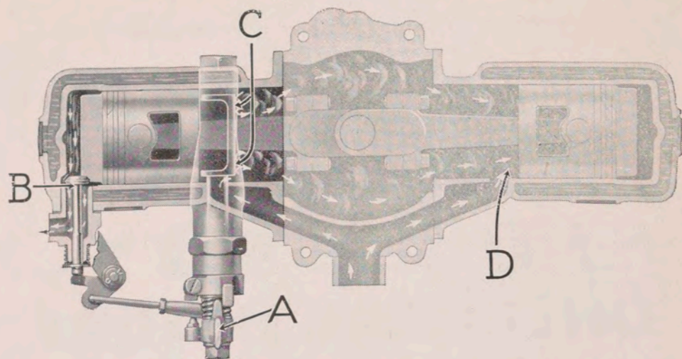
Sectional view of the Johnson power head showing action of Release Charger for positive, easy starting. Lever (A) opens valve (B) releasing compression and closing intake passage (C) in inactive cylinder. Entire charge (D) is forced into active cylinder. The released compression in the inactive cylinder increases the spark intensity in the active cylinder.
