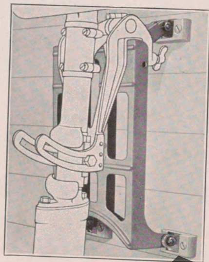
Close-up view showing the method of installation.
