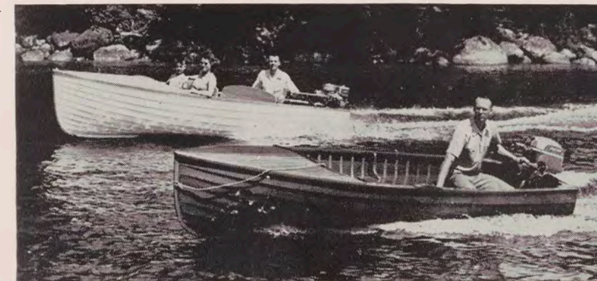
15 ft. Lapstrake Outboard—22 H.P. Motor—Background 13½ ft. Lapstrake Decked—10 H.P. Motor—Foreground
