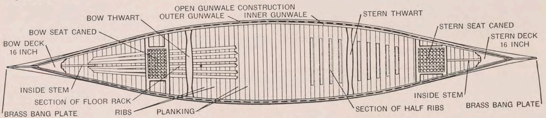
DIAGRAM of the "Old Town Canoe"
