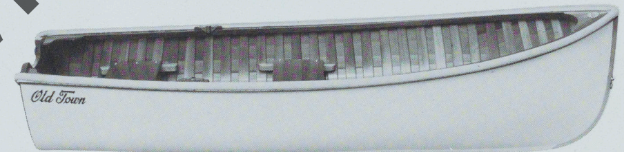
Wood dinghy: length 9'3"; width 49", depth 19"; bow height 26½"; weight 110 lbs.
