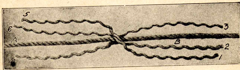
Fig. 9. Starting the Long Splice
