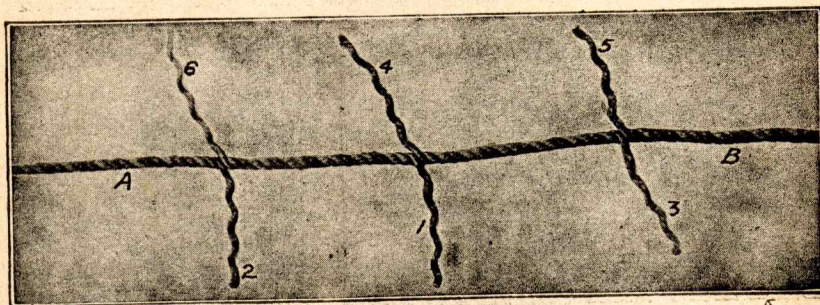
Fig. 10. Ready to Tie the Knots in the Long Splice. Ends 1, 2 and 3 Are from Rope A. Ends 4, 5 and 6 Are from Rope B
