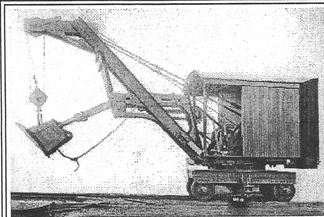
Captain Thew tried to develop a faster way to unload his ship on the Lakes. He came up with a gear system that allowed the shovels to rotate around all 360 degrees. The system had never worked before, but he made it work. After retiring from being captain of ships, he and others established the Thew Shovel Company of Lorain. This picture depicts one of the early models that were made in Lorain.
